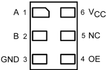
Figure 3. MicroPak™ (Top Through View)
