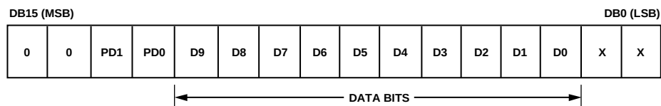
Figure 40. AD5612 Input Register Contents
