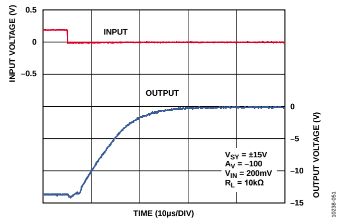
Figure 47. Negative Overload Recovery
