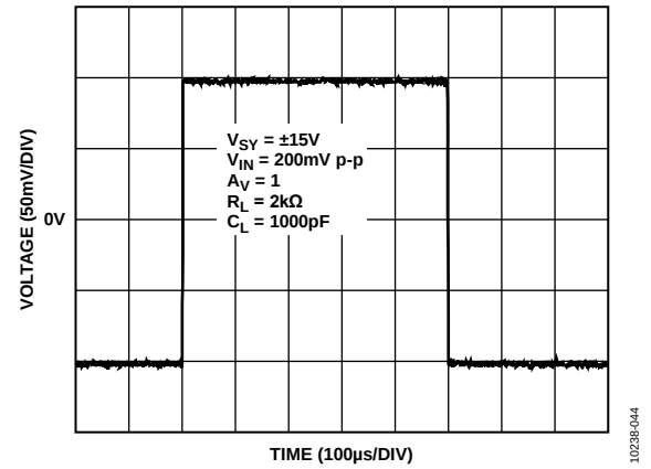
Figure 45. Small Signal Transient Response
