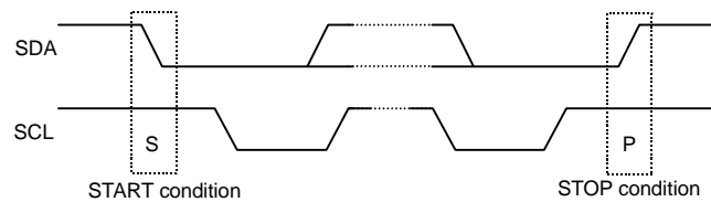
Figure 54. START/STOP condition (I 2 C format)
