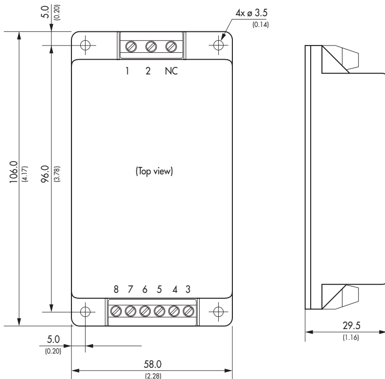
TMT 30C triple output models and TMT 30252C (screw terminal block)
