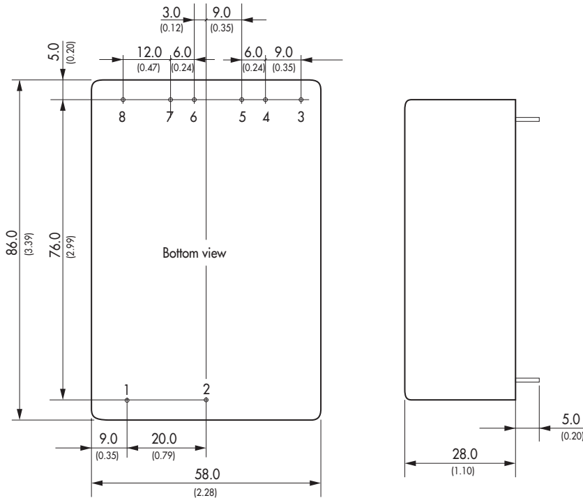
TMT 30 triple output models and TMT 30252 (solder pins)
