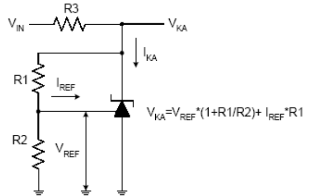
Test Circuit 5 for V_{KA} > V_{REF}
