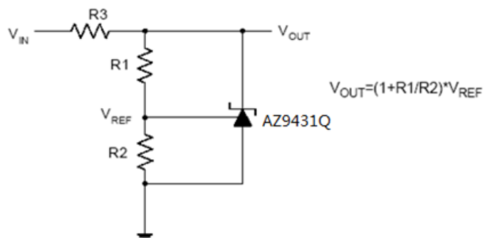
Shunt Regulator
