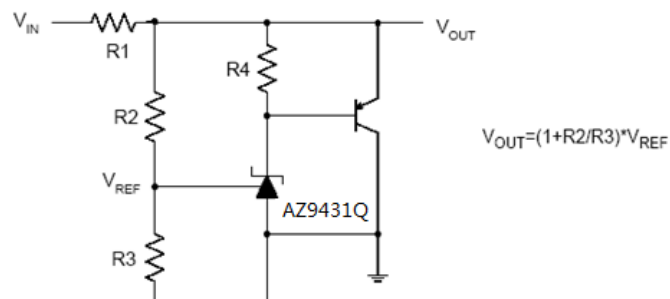
High Current Shunt Regulator
