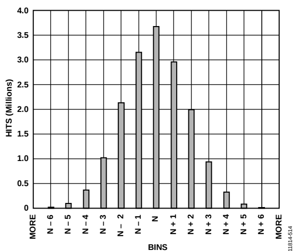
Figure 55. Input Referred Noise Histogram with 2.6 GSPS
