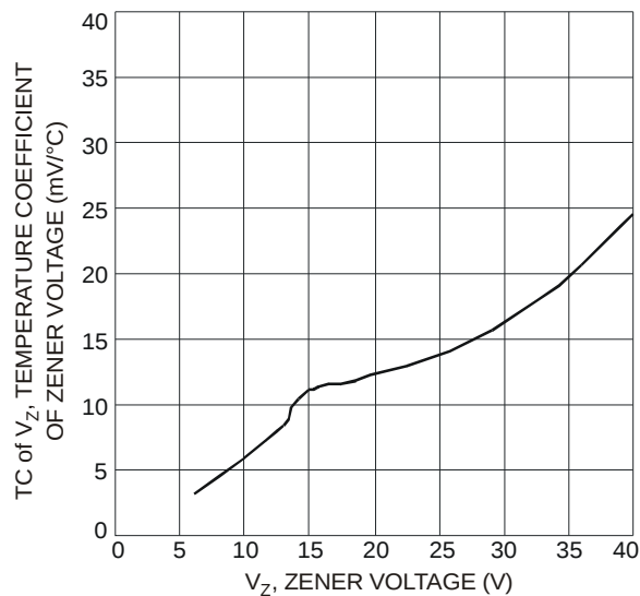
Fig. 2 Typical Temperature Coefficient of Zener Voltage vs. Zener Voltage
