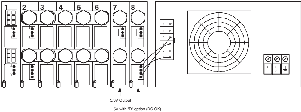
Figure 17 Output sequencing wire interconnect
