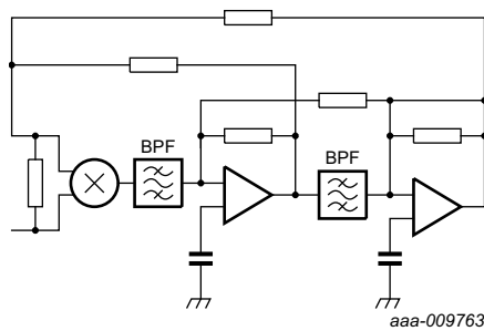
Fig 9. Second limiter and quadrature detector
