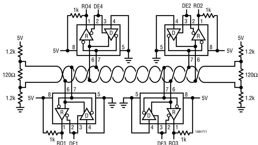
Figure 11. Transmit "0" CDMA Application
