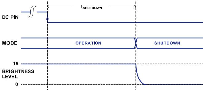
Figure 3. Shutdown Timing
