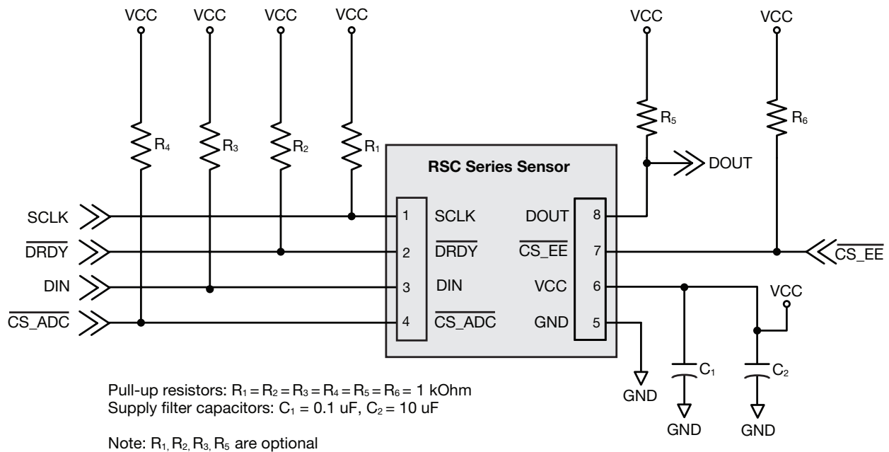
Figure 7. Recommended Circuit
