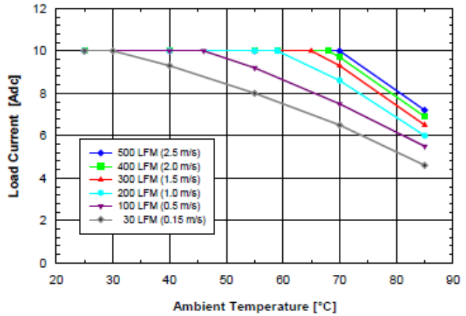
Fig. 5.0V.4: Available load current vs. ambient air temperature and airflow rates for SQ48S10050 converter mounted horizontally with Vin = 48V, air flowing from pin 3 to pin 1, and maximum FET temperature ≤ 120°C.
