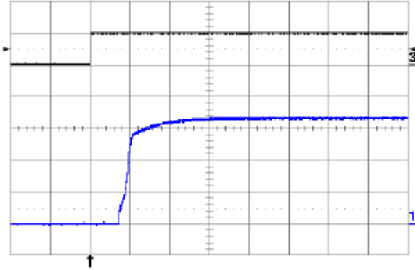
Fig. 3.3V.9: Turn-on transient at full rated load current (resistive) with no output capacitor at V_{in} = 48\text{ V} , triggered via ON/OFF pin. Top trace: ON/OFF signal (5 V/div.). Bottom trace: output voltage (1 V/div.). Time scale: 2 ms/div.
