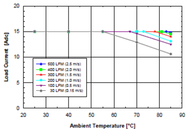
Fig. 2.5V.4: Available load current vs. ambient air temperature and airflow rates for SQ48S15025 converter
