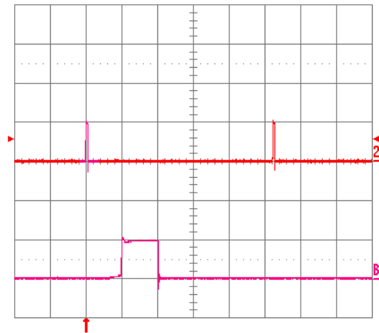
Fig. 1.5V.18: Load current (top trace, 20 A/div., 20 ms/div.) into a 10 m\Omega short circuit during restart, at V_{in} = 48 V. Bottom trace (20 A/div., 1 ms/div.) is an expansion of the on-time portion of the top trace.
