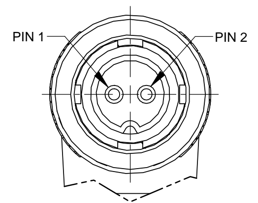
EN2C2M20 VIEWED FROM FRONT MATING SIDE OF CONNECTOR SCALE 3 : 1
