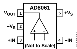
Figure 4. 5-Lead SOT-23 (RJ)
