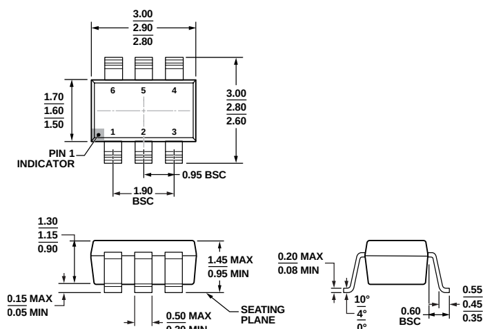
Figure 60. 6-Lead Small Outline Transistor Package [SOT-23] (RJ-6)
