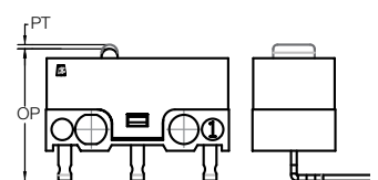
OP FROM TERMINAL (FOR TYPE 50 & 60 TERMINAL)
