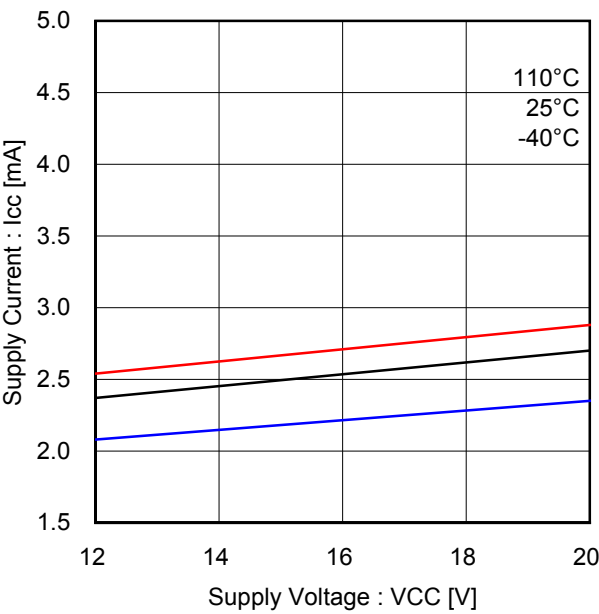
Figure 14. Quiescent Current (Low Side Drivers)
