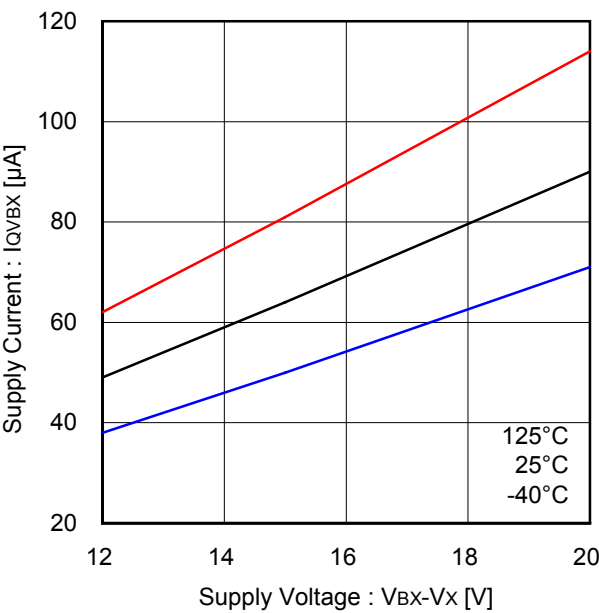
Figure 16. Quiescent Current (High Side Driver, Each Phase)
