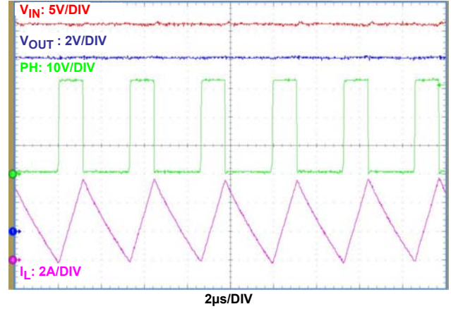
FIGURE 13. FORCED PWM MODE, V_{IN} = 36V , V_{OUT} = 12V , I_{OUT} = 2.5A , L = 4.7\mu H , C_{OUT} = 98\mu F , f_{SW} = 300kHz
