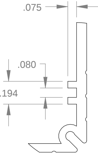
DETAIL C
