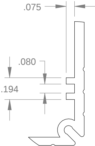
DETAIL C
