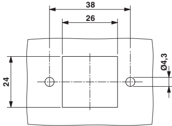
Panel cutout
