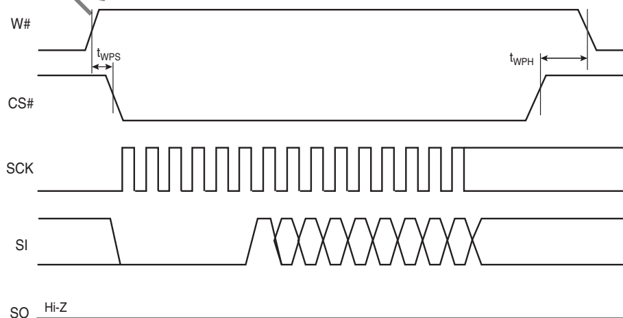
Figure 48. Write Protect Setup and Hold Timing during WRR when SRWD = 1
