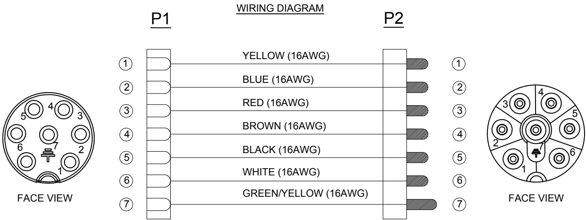
FEMALE CONNECTOR PLUG
