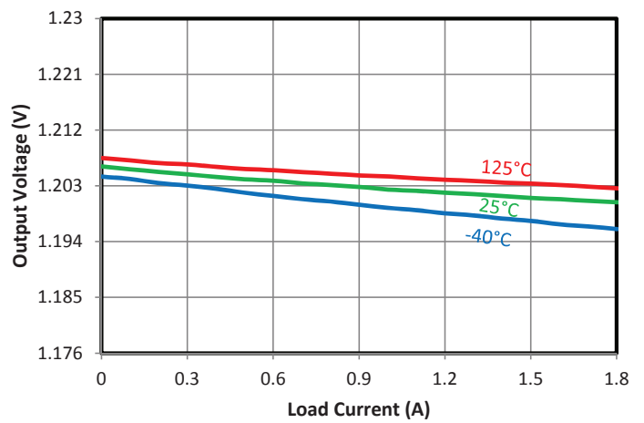
Load Regulation, V_{out}=1.2V
