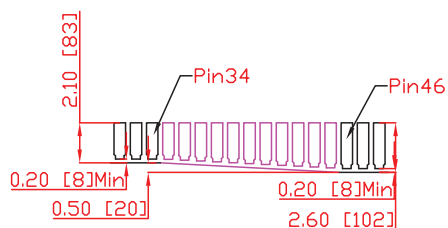
Detail C
