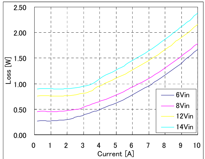
Fig-3.3V-3: Power Loss vs. load current and input voltage for V_{out}=3.3V . Airflow rate=200 LFM (1m/s) and T_a=25^{\circ}C .
