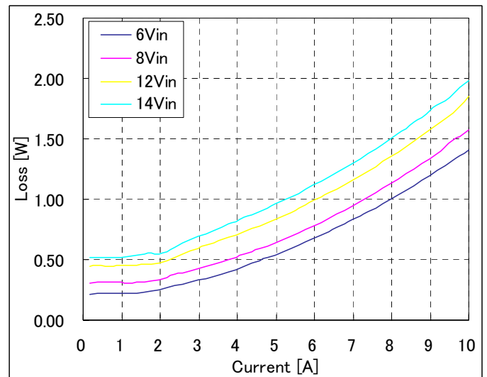
Fig-1.8V-3: Power Loss vs. load current and input voltage for V_{out}=1.8V . Airflow rate=200 LFM (1m/s) and T_a=25^{\circ}C .
