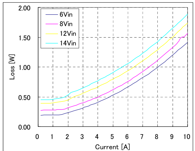
Fig-1.5V-3: Power Loss vs. load current and input voltage for V_{out}=1.5V . Airflow rate=200 LFM (1m/s) and T_a=25^{\circ}C .
