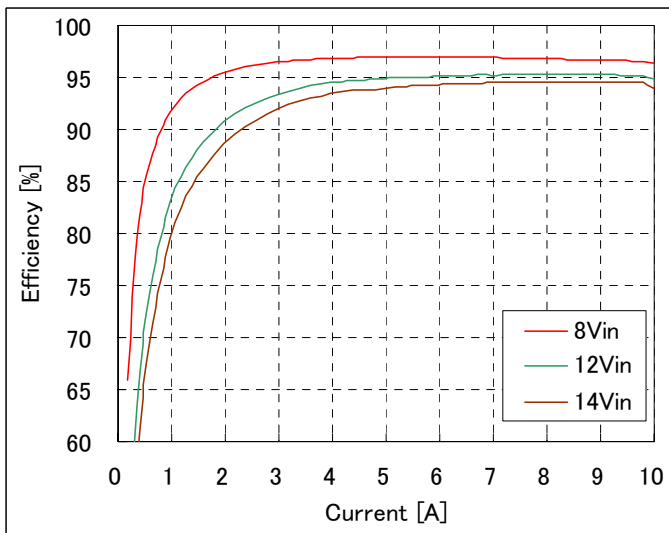
Fig-5.0V-2: Efficiency vs. load current and input voltage for V_{out}=5.0V . Airflow rate=200 LFM (1.0 m/s) and T_a=25^{\circ}C .
