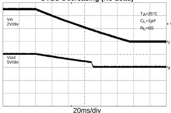
UVLO Decreasing (No Load)
