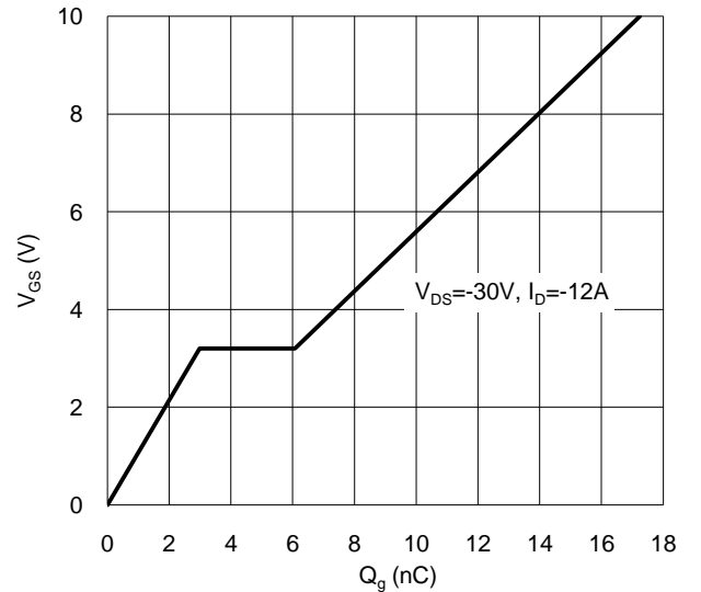
Figure 12. Gate Charge
