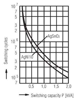
Mechanical life
