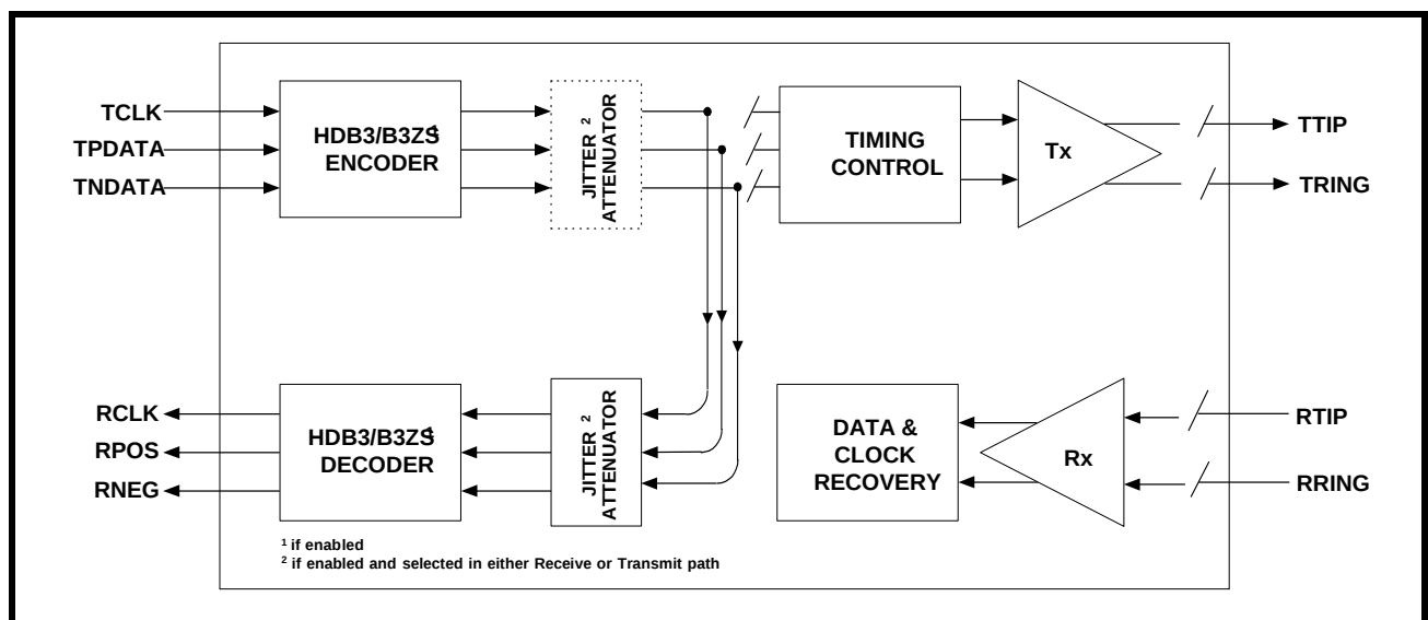
FIGURE 27. DIGITAL LOOPBACK
