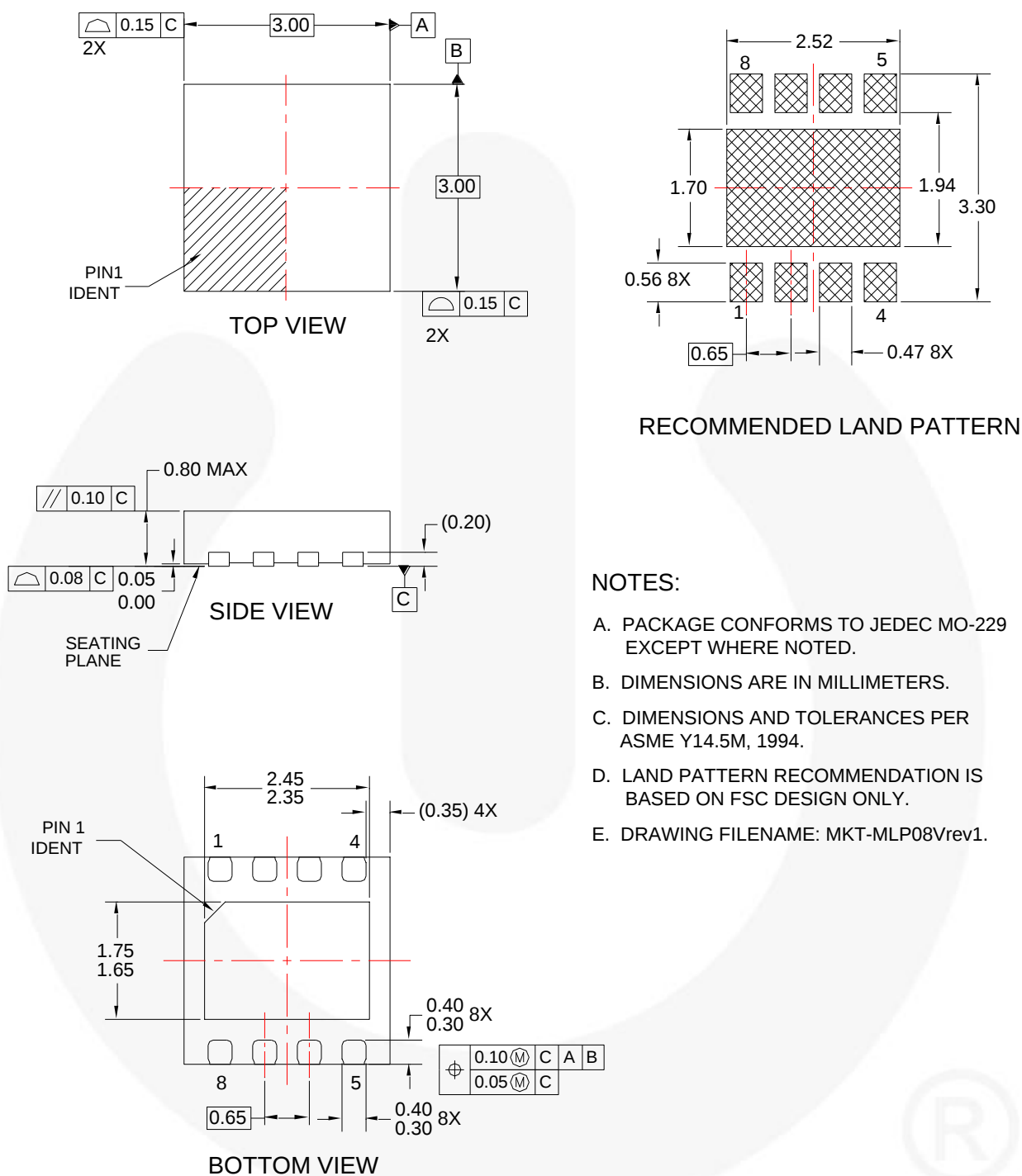
Figure 47. 8-Lead, 3x3 mm Molded Leadless Package (MLP)
