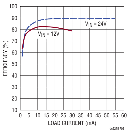
Figure 3. Efficiency vs Load
