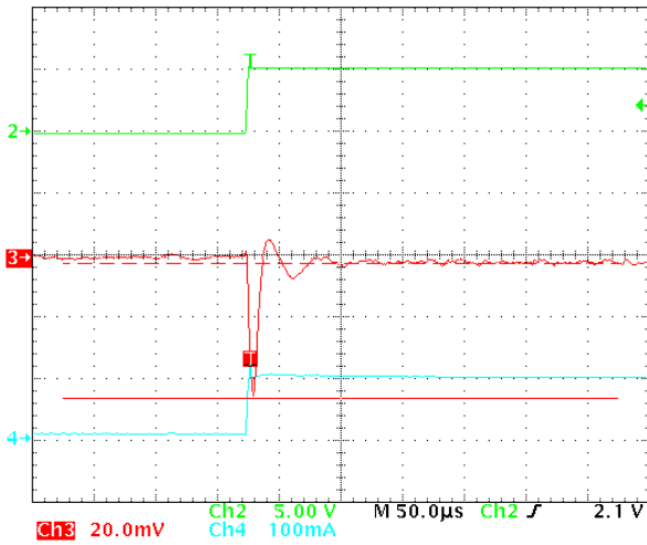
Figure 17. 10 mA to 100 mA Load Transient in 1 \mu\text{s} ( V_{IN} = 3.6 \text{ V} , V_{OUT} = 1.2 \text{ V} , Temperature = 25°C)
