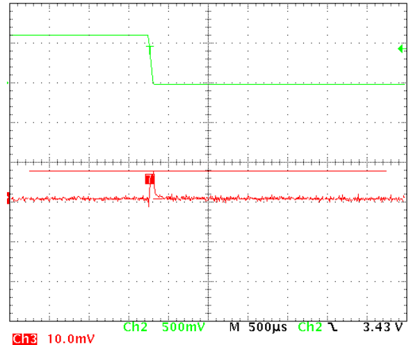
Figure 20. 3.6 V to 3.0 V Line Transient, Fall = 50 \mu\text{s} ( V_{IN} = 1.2 \text{ V} , I_{OUT} = 100 \text{ mA} , Temperature = 25°C)
