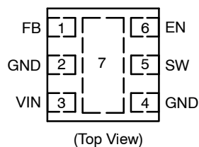
Figure 4. Pin Connections – UDFN6
