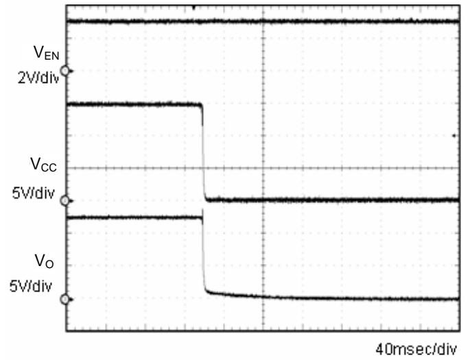
Fig.6 OFF sequence 1 Co=1μF
