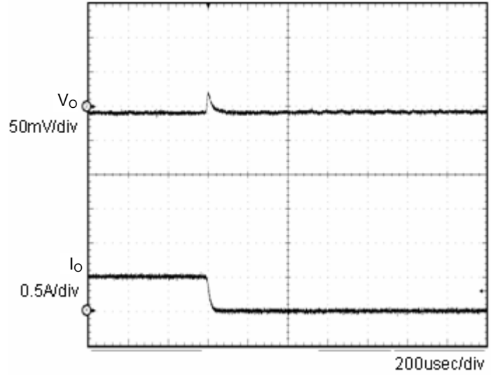
Fig.4 Transient Response (0.5→0A) Co=1μF
