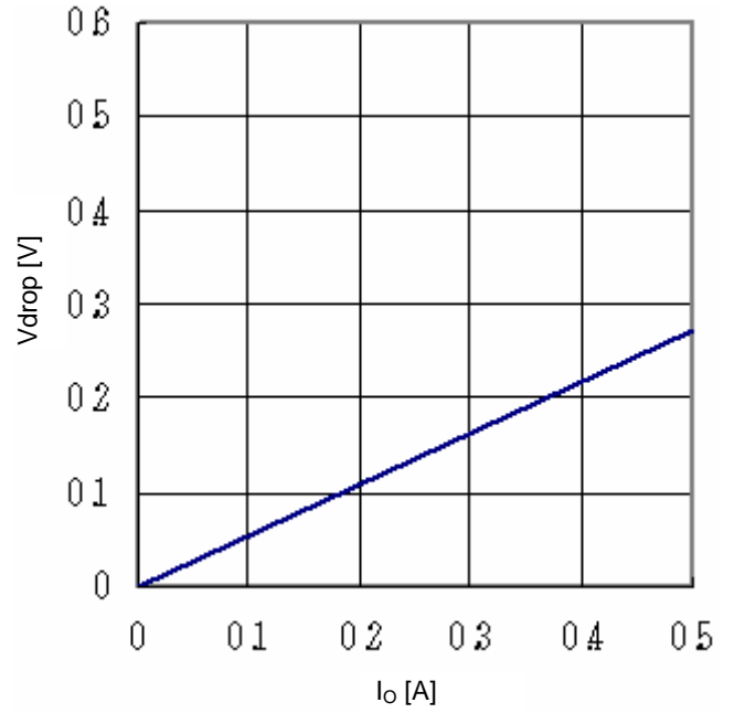
Fig.24 Minimum dropout Voltage 4 (V CC =8V、Ta=25°C)
