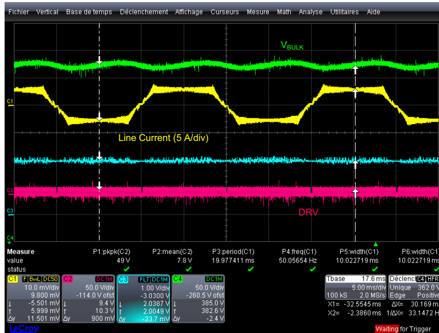
Figure 14. Over-Current Situation (85 V, 0.5 A Load Current)
