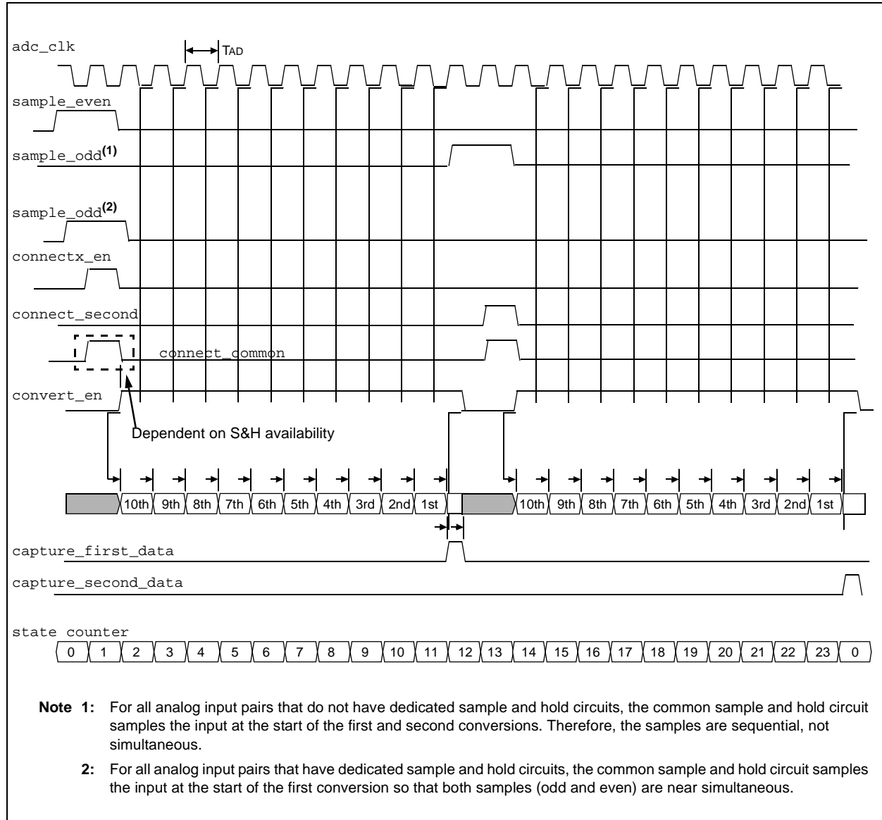
FIGURE 16-4: DETAILED CONVERSION SEQUENCE TIMINGS, SEQSPAMP = 1
