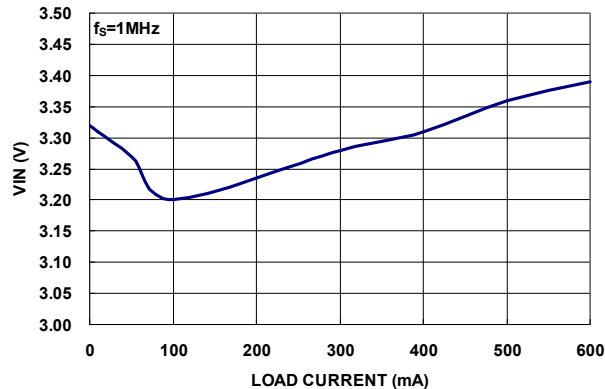
(a) V_{OUT}=3.3V
