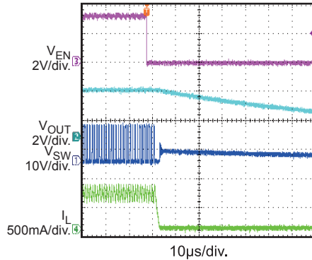
Shutdown through EN I_{OUT}=0.6A
