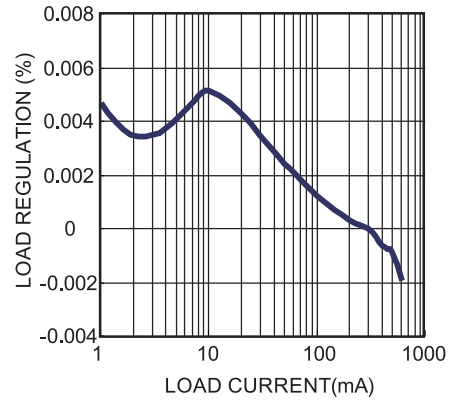
Load Regulation
