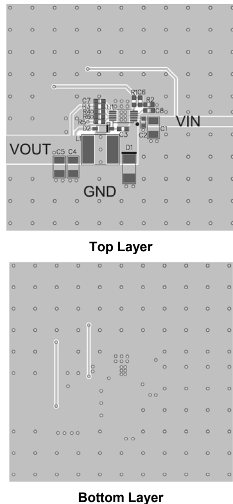
Figure 4: Recommended PCB Layout
