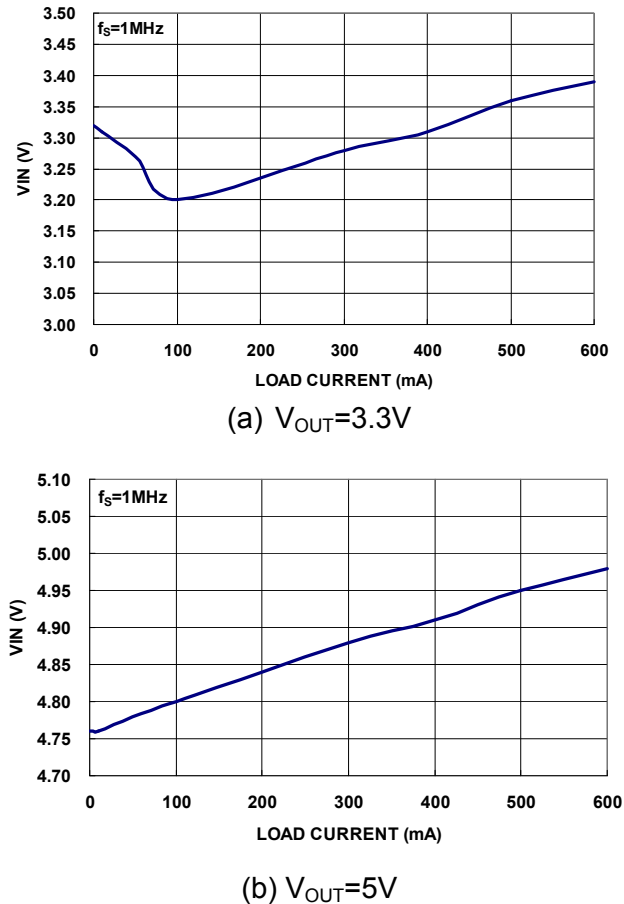
Figure 3 : Minimum Input Voltage vs. Load Current
