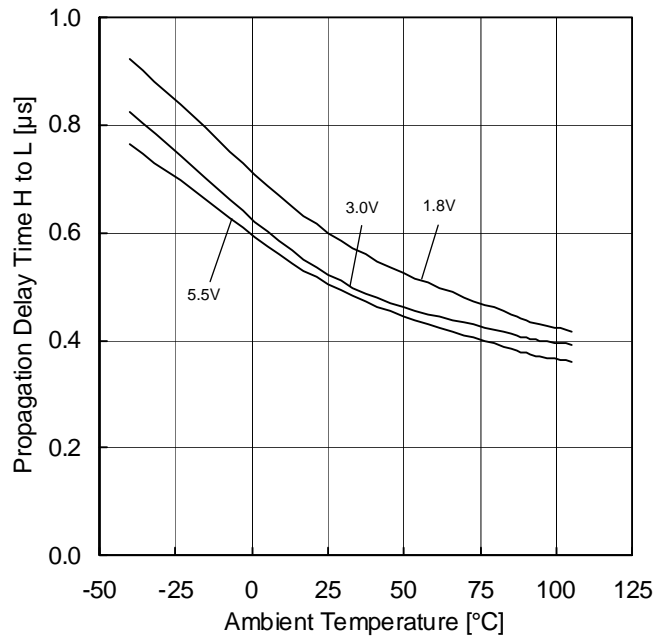
Figure 20. Propagation Delay Time H to L vs Ambient Temperature ( R_L=10k\Omega , V_{RL}=3V , C_L=15pF I_N=-1.5V , 100mV Overdrive)
