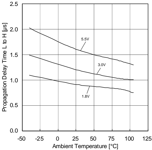
Figure 19. Propagation Delay Time L to H vs Ambient Temperature ( R_L=10k\Omega , V_{RL}=3V , C_L=15pF I_N=-1.5V , 100mV Overdrive)
