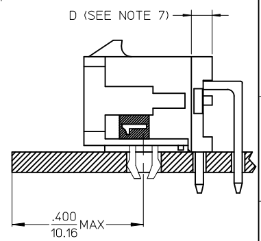
LOCATION DETAIL SEE NOTE #8
