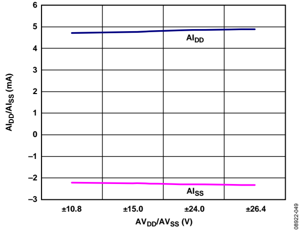
Figure 47. A_{I_{DD}}/A_{I_{SS}} vs. A_{V_{DD}}/A_{V_{SS}} , V_{OUT} = 0\text{ V}
