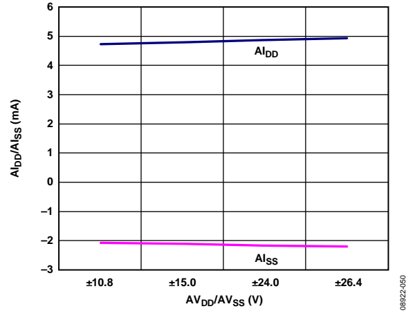
Figure 48. A_{I_{DD}}/A_{I_{SS}} vs. A_{V_{DD}}/A_{V_{SS}} , I_{OUT} = 0\text{ mA}
