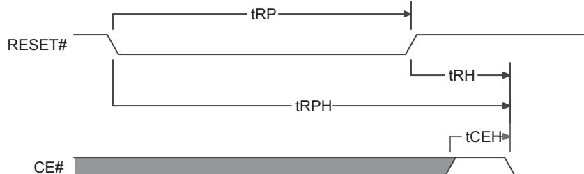
Figure 21. Hardware Reset
