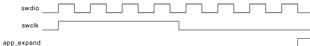
Figure 6.3. APP Expansion
