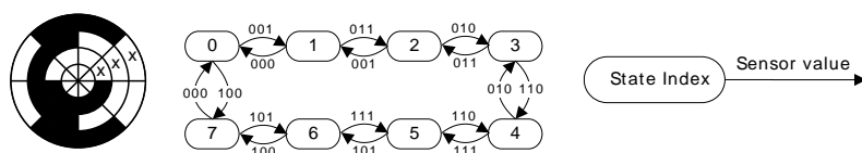
Figure 25.13. FSM example 1
