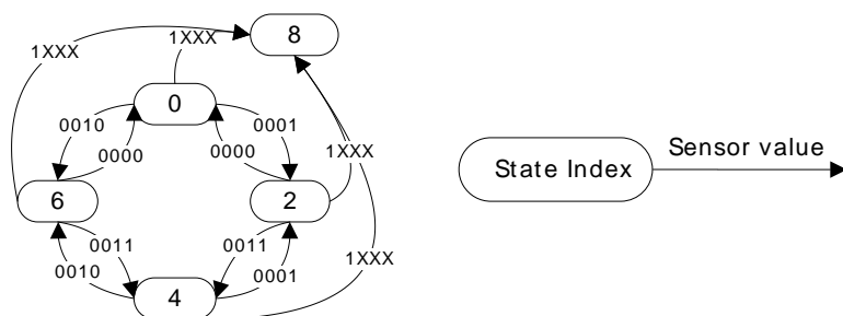
Figure 25.14. FSM example 2
