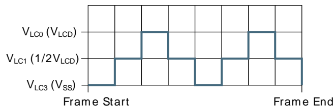
Figure 33.6. LCD 1/2 Bias and Duplex Multiplexing - LCD_COM1
