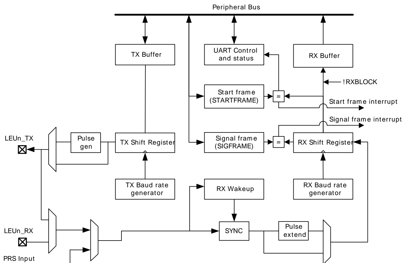
Figure 19.1. LEUART Overview
