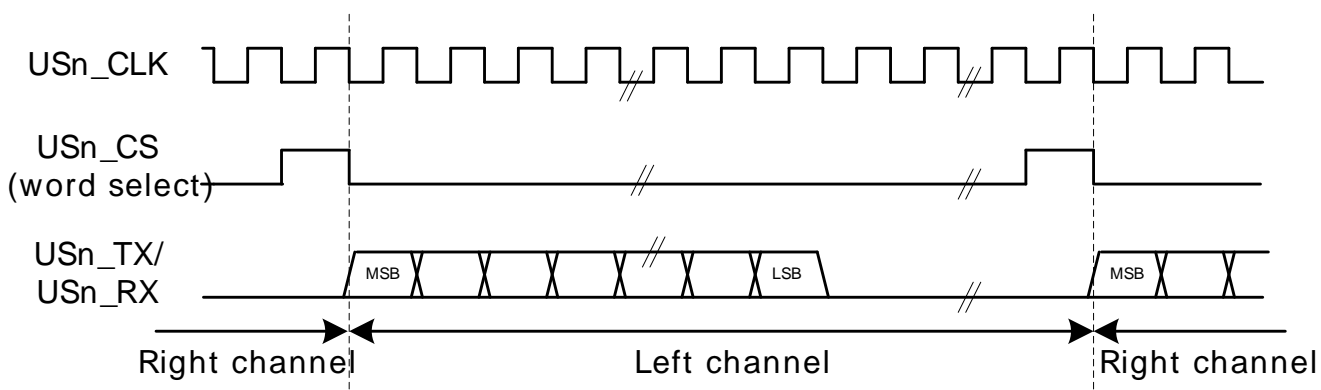
Figure 17.20. USART Mono I2S waveform
