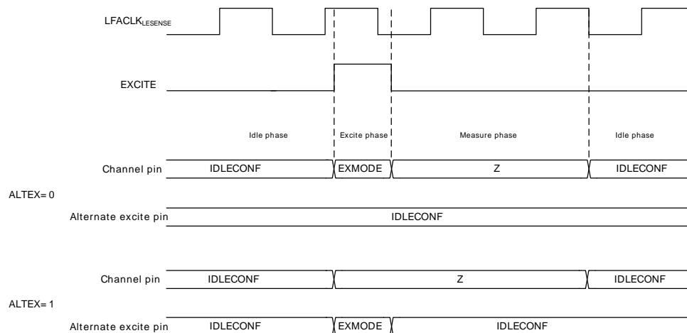
Figure 25.4. Pin sequencing
