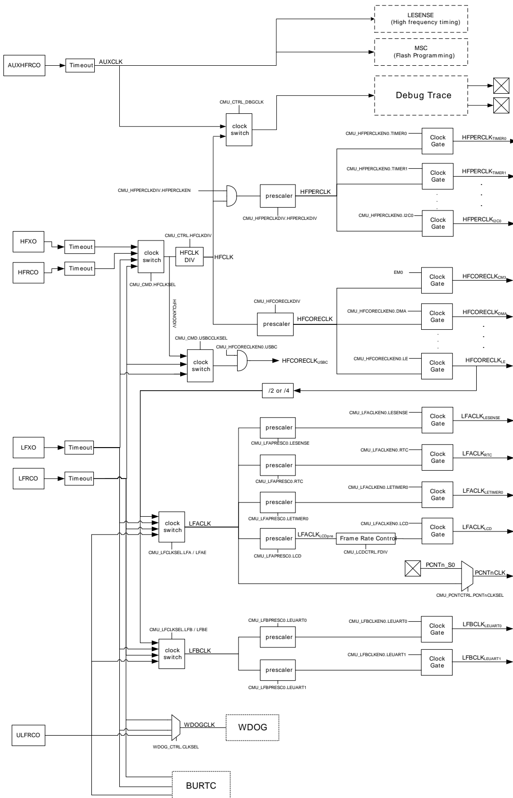
Figure 11.1. CMU Overview
