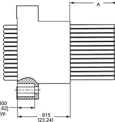
Plug Assembly
