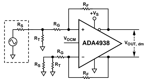
Figure 60. ADA4938-x Configured for Unbalanced (Single-Ended) Input
