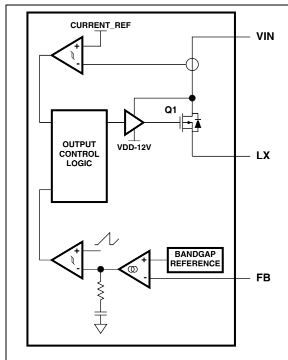
FIGURE 4-1: SMPS Functional Block Diagram.
