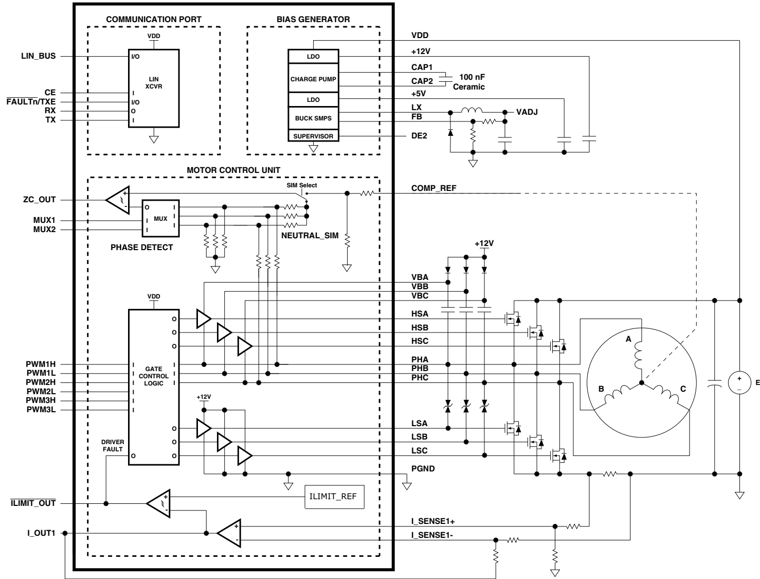
Typical Application Circuit – MCP8025
