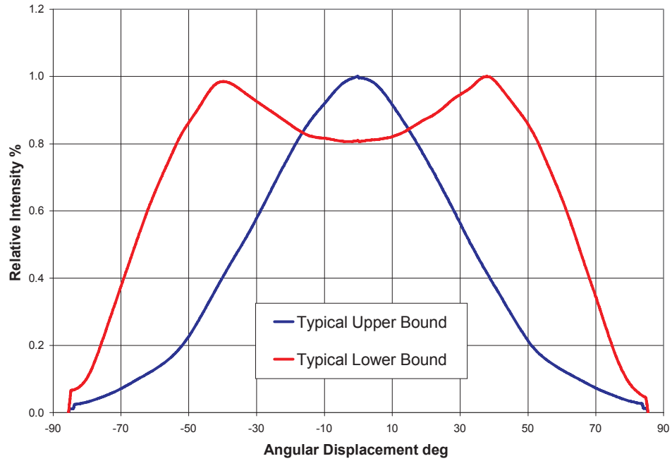
Figure 19: Typical Representative Spatial Radiation Pattern for Green and Royal Blue Lambertian.
